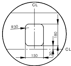
DETAIL C SCALE 1 : 10 S30 window template W12601
